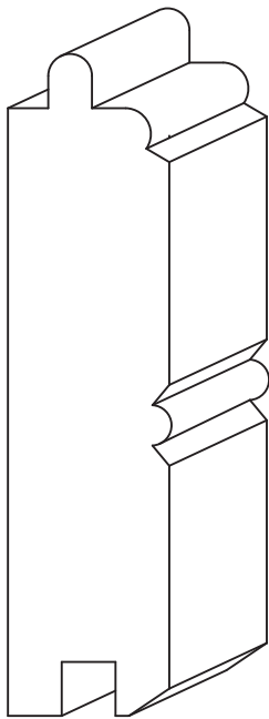
KCW-3801 3/4" x 3-1/8" BEADED CEILING
