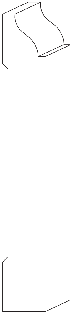
KCW-618B 3/4" x 5 1/4"
