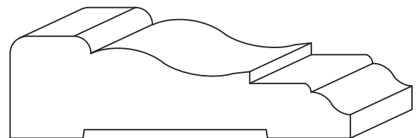
KCW-347 3/4" x 2-9/16"
