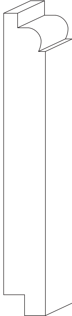
KCW-3702 3/4" x 5 1/2" BEADED SHIPLAP
