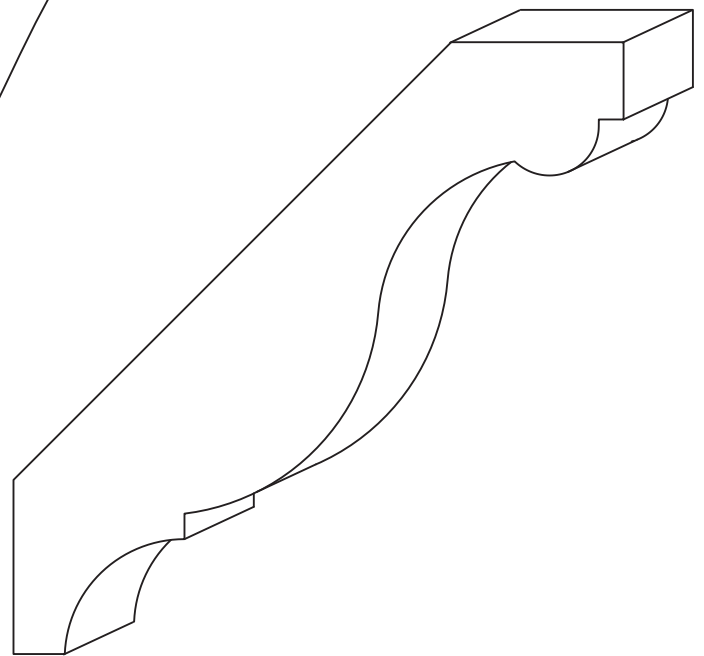
KCW-1819 1" x 4 1/2"
