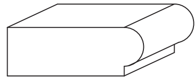
KCW-3505 1/2" x 1-3/8"
