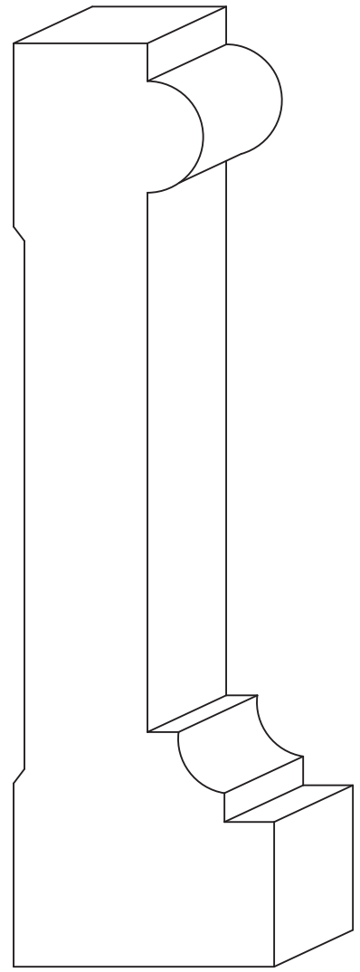
KCW-641 1 1/2" x 5-5/16"
