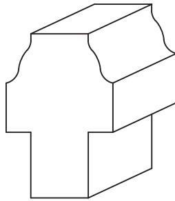
KCW-4401 7/16" x 1 1/4"
